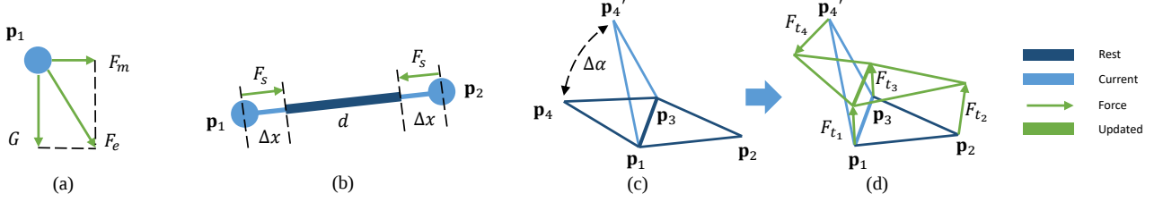
Figure 4. Simulation forces in our system. (a) Resultant external force F_e on vertex \mathbf{p}_1 , which include gravity G and other external force F_m ; (b) Stretching force F_s between vertex \mathbf{p}_1 and \mathbf{p}_2 , where d is the rest length of the stretching spring and \Delta x is half of the length difference between rest length and current length; (c) The rest status and delta angle \Delta\alpha of current status of torsion spring. (d) Torsion force on the 4 vertices ( \mathbf{p}_1 , \mathbf{p}_2 , \mathbf{p}_3 and \mathbf{p}_4 ) of the two connected triangles and the updated position.
