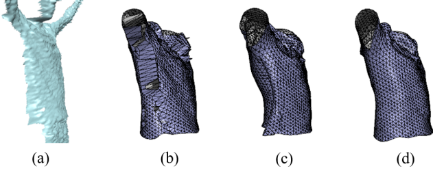
Figure 5. Illustration of iterative depth fitting. From left to right: depth input (a), result of direct depth fitting (b), iterative depth fitting without (c) and with (d) smooth blending.
